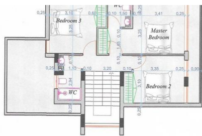
1. First Floor 1:100
